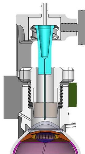
Section view of the Robo-VIREC
