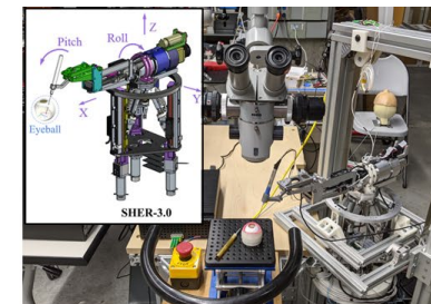
Robot-Assisted Retinal Surgery
