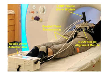
Robots for MRI-guided Percutaneous Interventions
