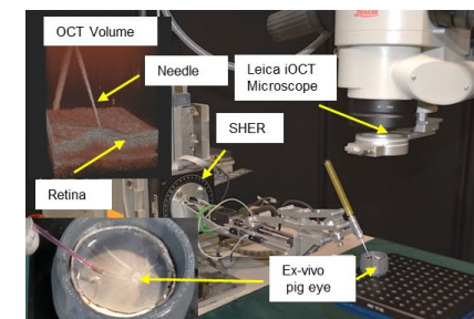
OCT-guided Robot-Assisted Retinal Surgery
