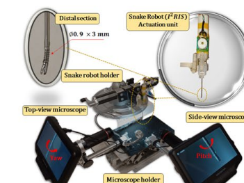
Intraocular Snake-like Robot
