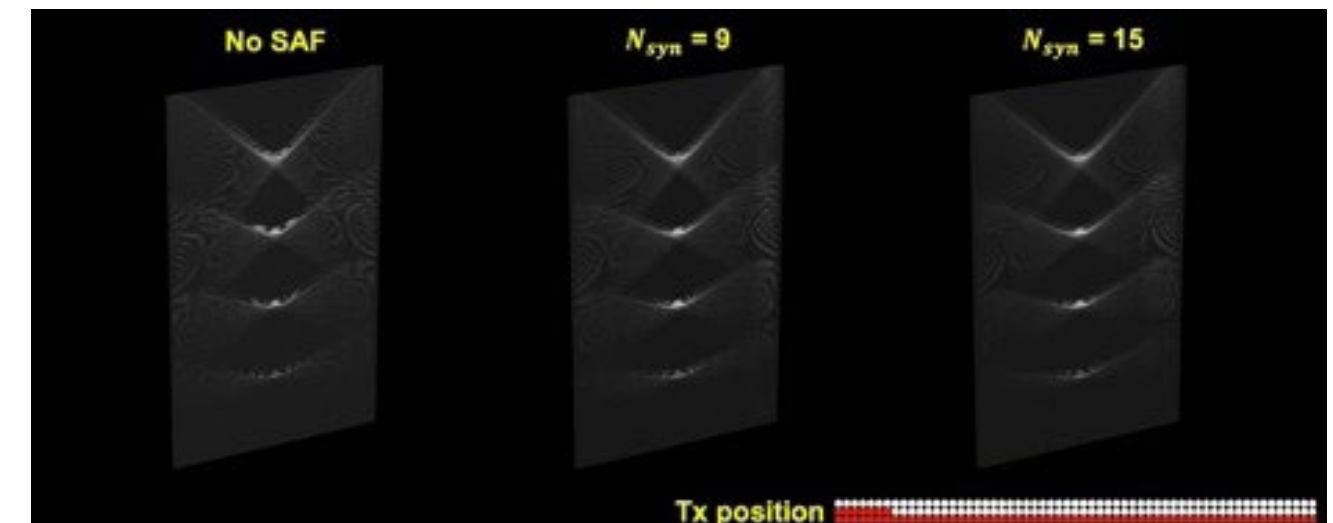
Optimization of imaging performance. The three volumetric images show the ncLUS imaging performance based on different imaging parameters of the synthetic aperture focusing (SAF).
