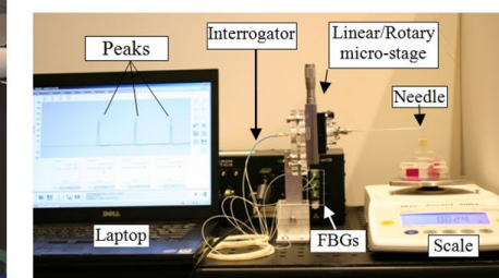
Real-Time Shape Sensing for Flexible Needles
